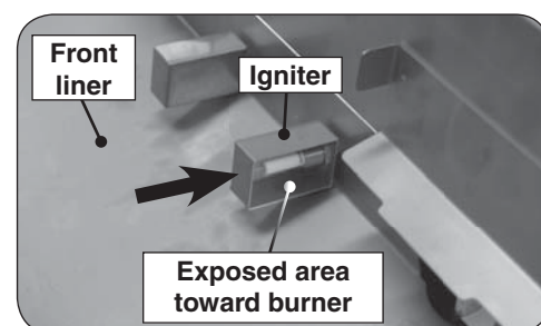
Fig. 2-6 Install igniters
