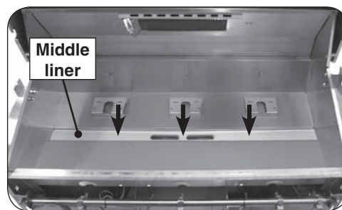
Fig. 1-3 Install middle liner
