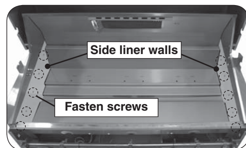
Fig. 2-4 Install side liner walls
