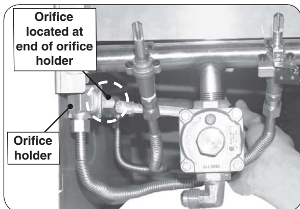
Fig. 21-3 Orifice location
