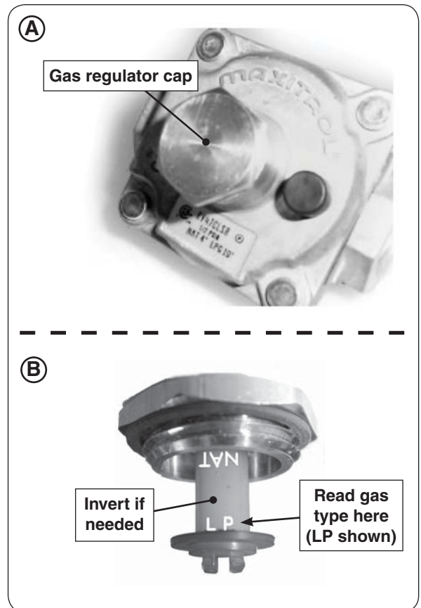
Fig. 20-1 Convert regulator
