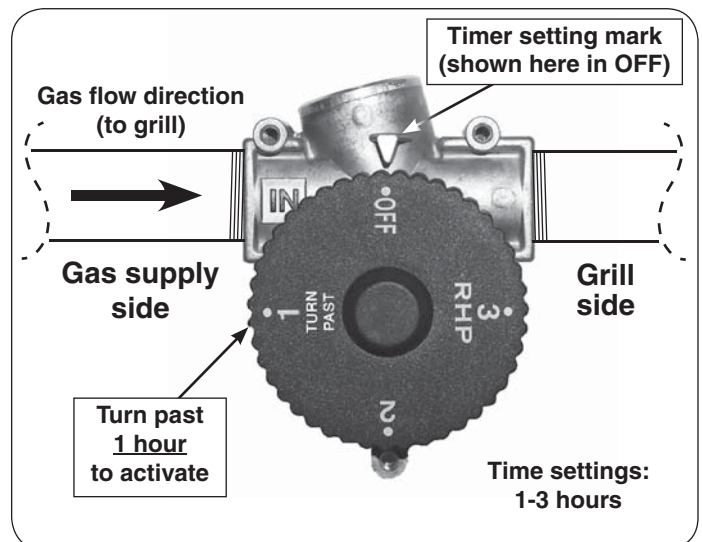
Fig. 1-2 Horizontal setup
