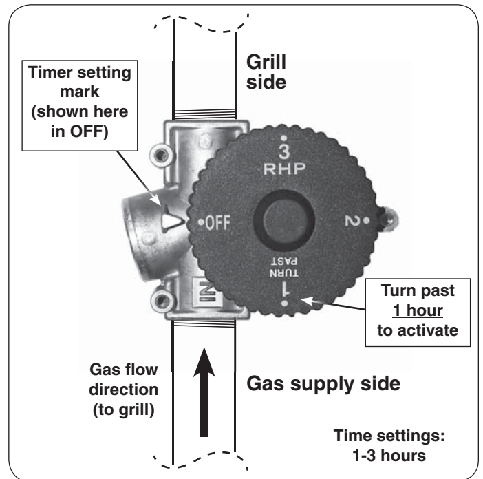
Fig. 1-1 Vertical setup
