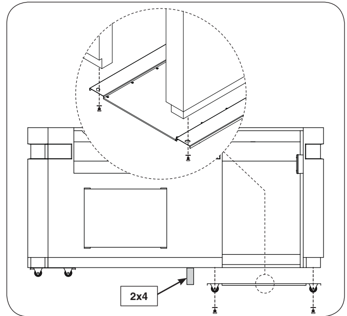
Fig. 4-1 Install right wheel assembly
