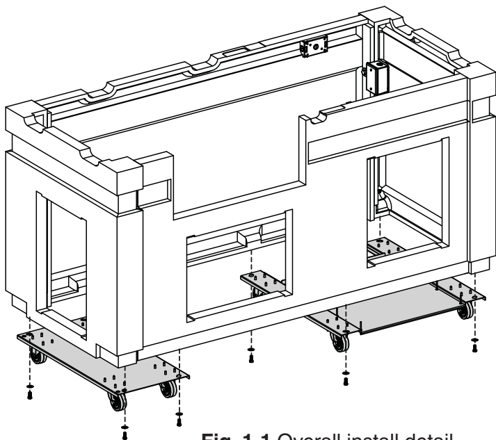
Fig. 1-1 Overall install detail
