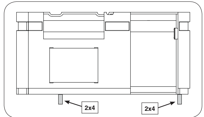
Fig. 3-2 Place 2x4's under island enclosure
