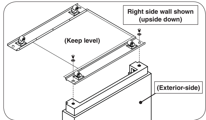
Fig. 2-2 Install right wheel assembly to bottom of right side wall
