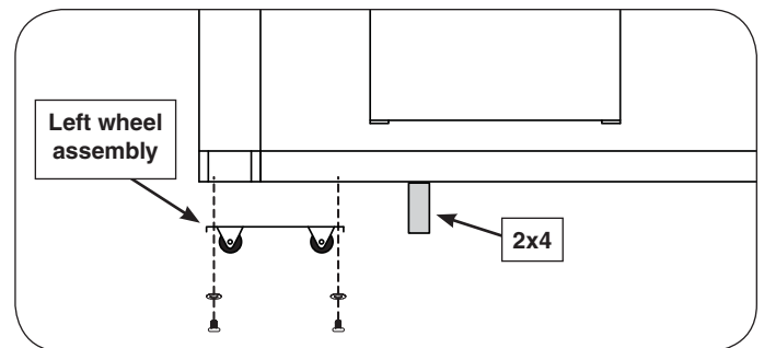
Fig. 3-4 Install left wheel assembly
