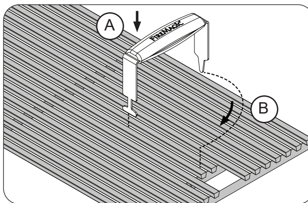
Fig. 24-2 Install cooking grids
