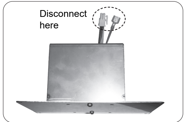
Fig. 41-2 Disconnect wire harness and groundwire (and power cord)
