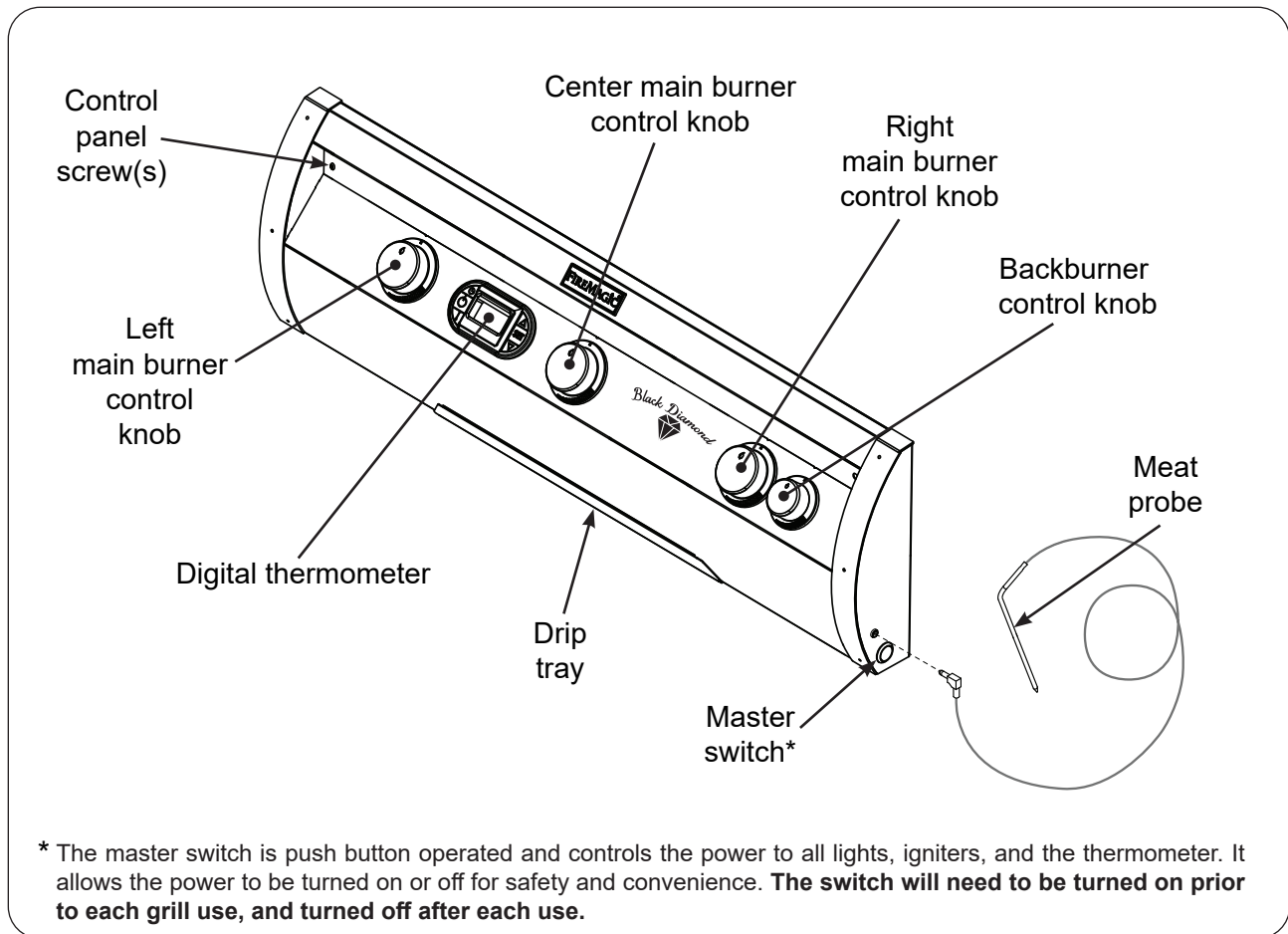
Fig. 27-1 H790i controls
