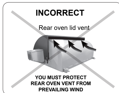
Fig. 15-4 Airflow direction - INCORRECT
