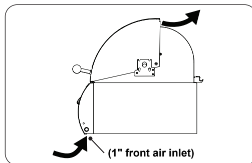
Fig. 15-2 Airflow diagram
