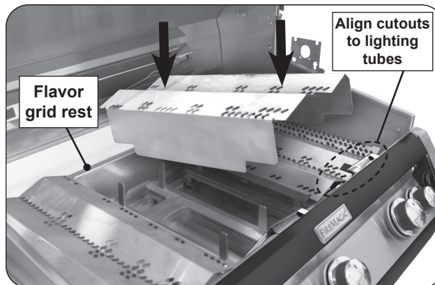
Fig. 24-1 Install flavor grids
