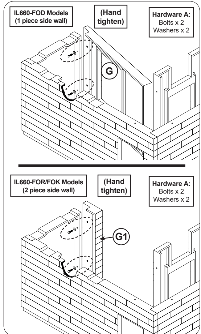
Fig. 12-3 Assemble side wall
