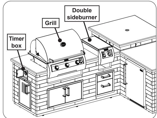
Fig. 18-3 Install grill, sideburner, and timer box
