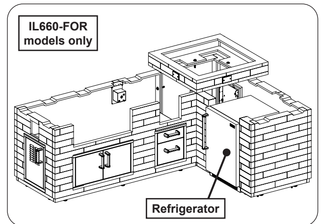
Fig. 17-2 Install refrigerator (if applicable)
