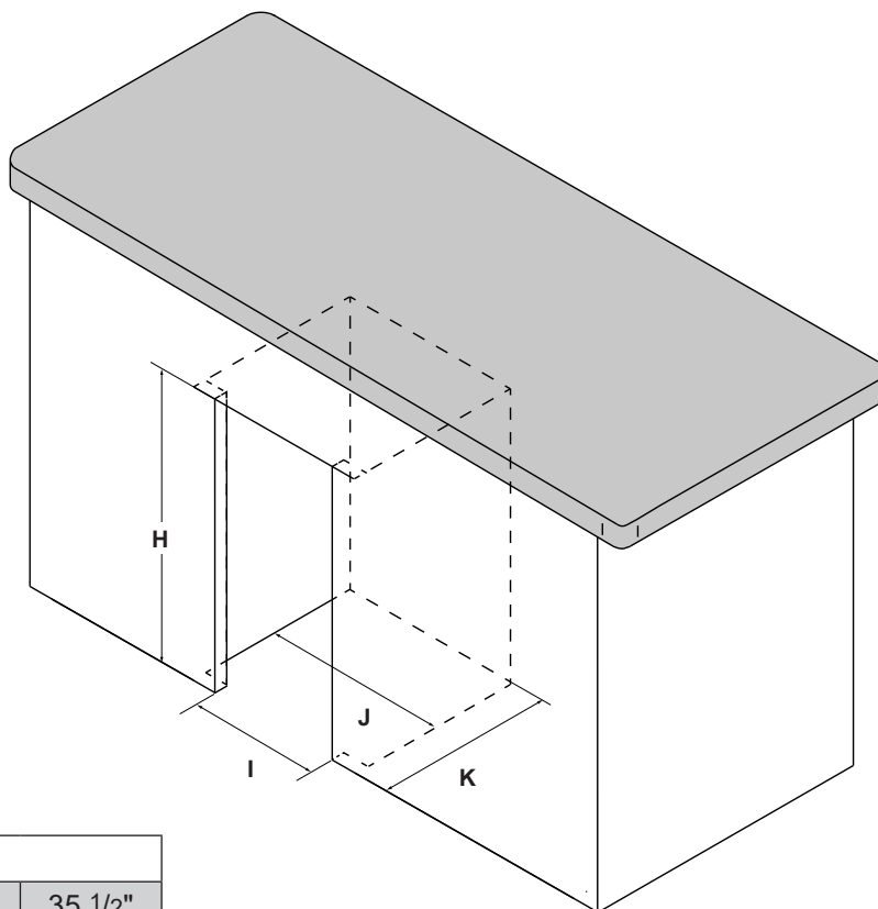
Fig. 6-2 Cut-out/ clearance dimensions diagram
