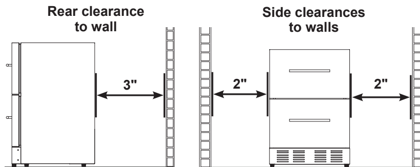
Fig. 4-2 Cut out wall clearances
