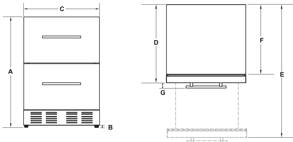
Fig. 6-1 Unit dimensions
