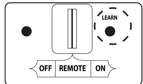
Fig. 13-1 Remote receiver sync detail
