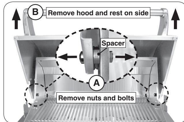
Fig. 2-2 Remove hood
