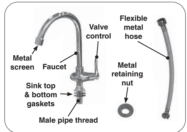
Fig. 1-1 Faucet detail
