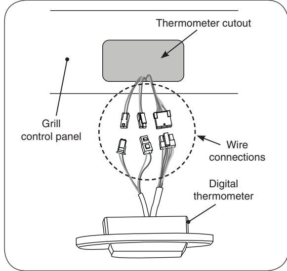
Fig. 1-1 Removing / connecting digital thermometer
