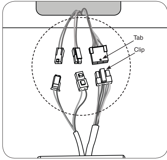
Fig. 1-2 Proper connections
