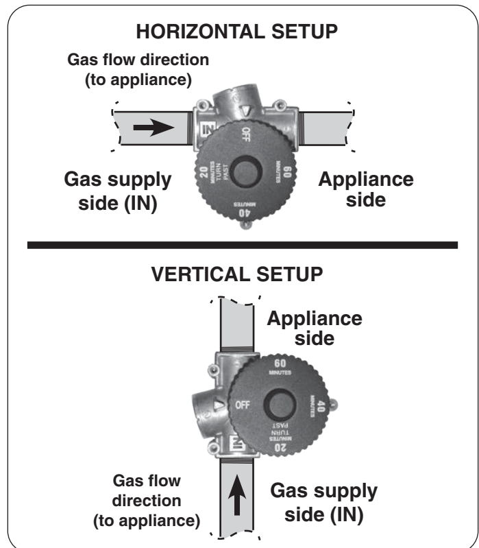
Fig. 1-2 Automatic timer shut-off valve installation detail
