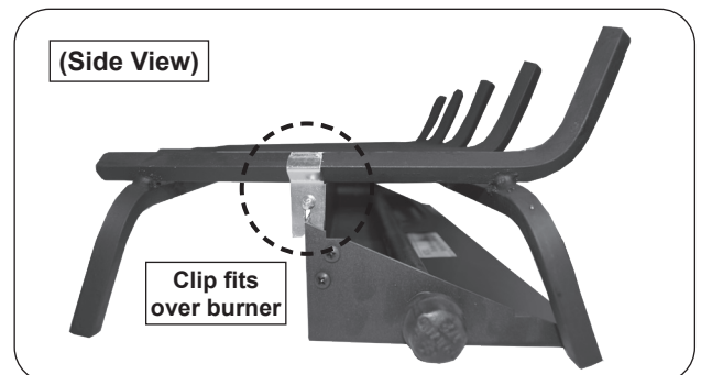
Fig. 11-3 Grate placement detail
