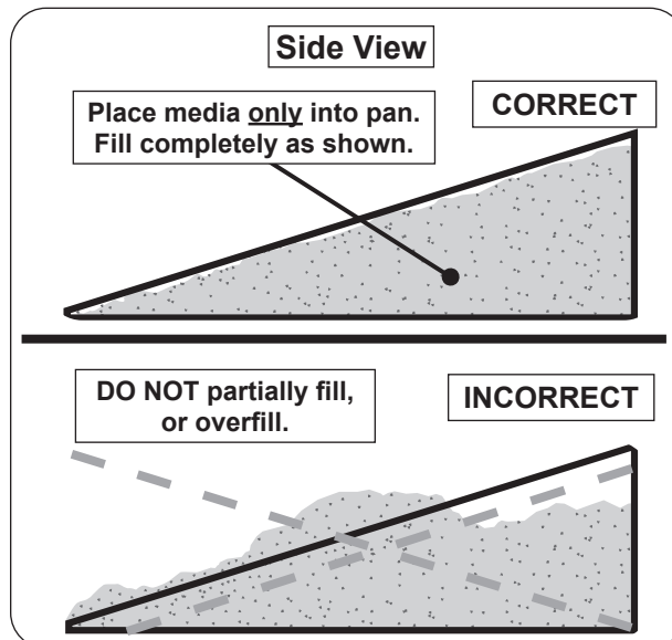
Fig. 12-2 Correct/Incorrect media placement (sand or vermiculite)
