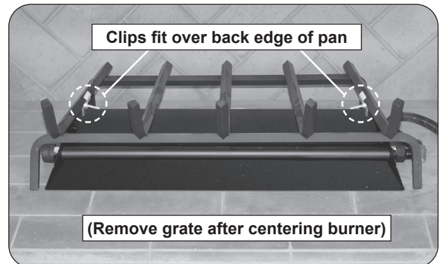
Fig. 11-2 Position grate
