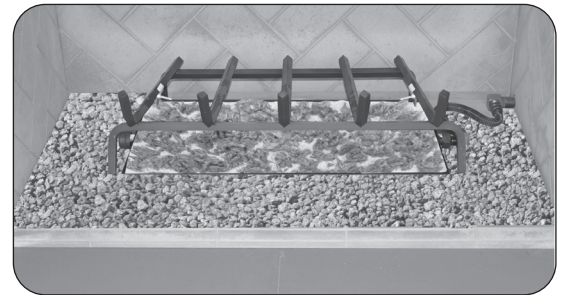
Fig. 13-3 Place grate
