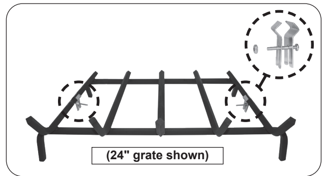
Fig. 11-1 Attach stabilizer clips to grate
