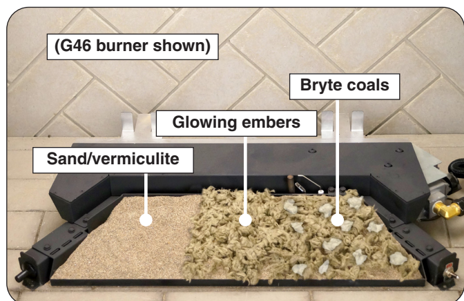
Fig. 2-1 Place burner pan media
