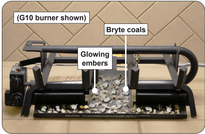
Fig. 2-3 Place burner pan media
